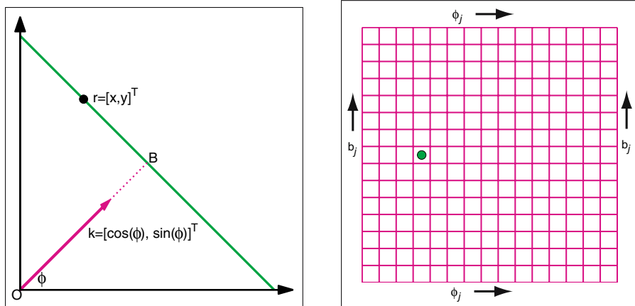
Fig. 10.33. (left) A common model of a line (green) to be used in the Hough transform of a line is given by the vector k and the perpendicular distance of the origin to the line, b = |OB| . (right) The discretized parameter space (\phi, b_j) is shown. Edges in the (x, y) space cast votes to cells in the (\phi_j, b_j) space
